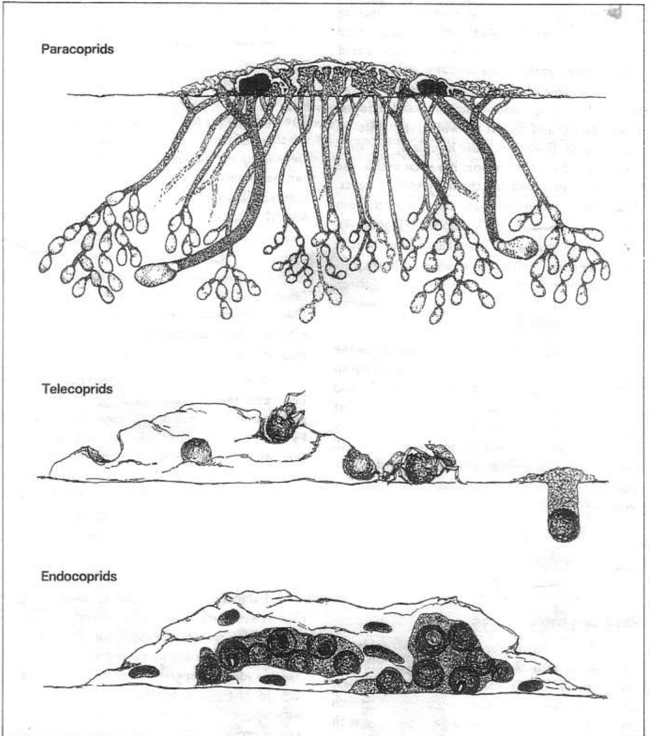
Figure 3: The most common dung beetles are the paracoprids, which bury dung beneath or around dung pads. The ball rollers or telecoprids carve chunks of dung out of the pad, knead them into balls and roll them away for burial. The least known and least effective beetles are the endocoprids, which build their nests inside dung pads during the dry warm periods when the other types are inactive.
